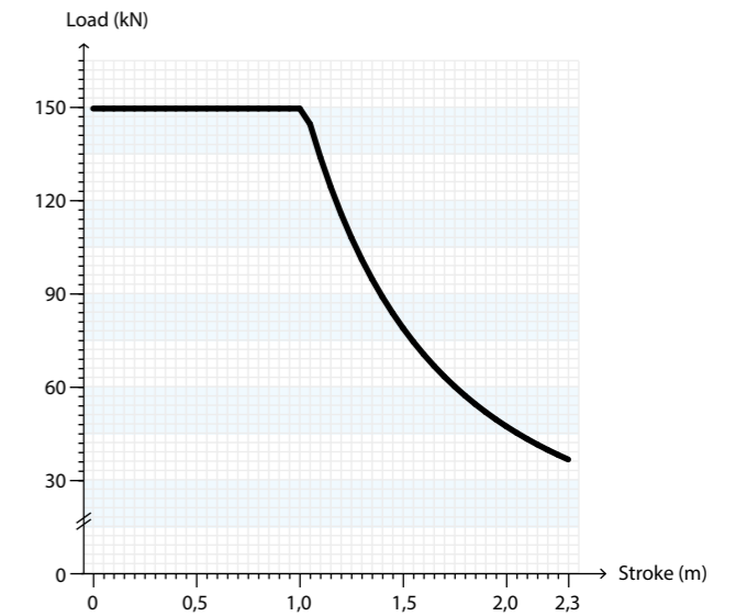
MAX. COMPRESSIVE FORCE TO AVOID BUCKLING
