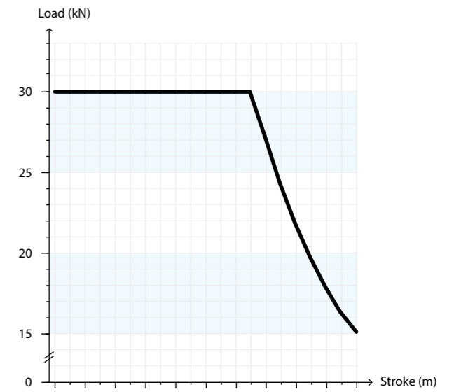
MAX. COMPRESSIVE FORCE TO AVOID BUCKLING
