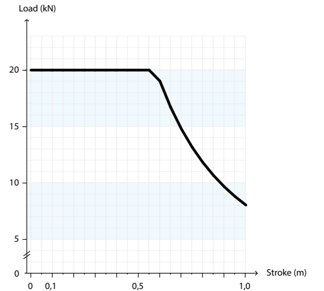
MAX. COMPRESSIVE FORCE TO AVOID BUCKLING
